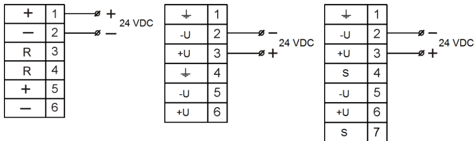
а) BC-07e-Eх-3(И)-24VDC
