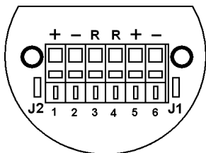
а) BC-07e-Eх-3(И)-24VDC
