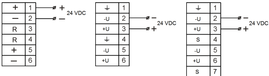
а) BC-07e-Ex-3(И)-24VDC
