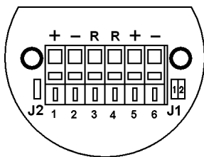
а) BC-07e-Eх-3(И)-24VDC
