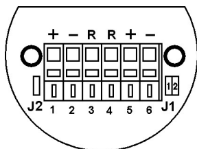
а) BC-07e-O-3(I)-24VDC
