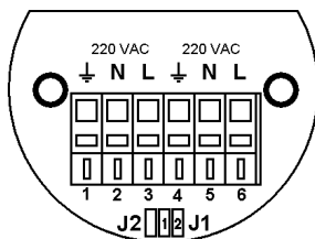
б) BC-07e-O-3(I)-230VAC
